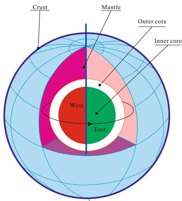
Figure 1. Schematic drawing showing the basic idea of the strong east-west asymmetry of the inner core due to melting of the inner-core boundary.
