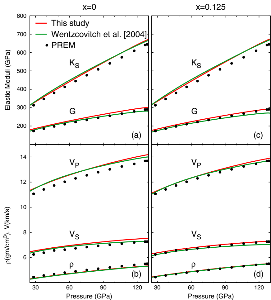
Figure 5. Elastic moduli ( K_S , G ), sound velocities ( V_P , V_S ), and density ( \rho ) for (Mg_{1-x}Fe_x^{2+})SiO_3 with (a, b) x=0 and (c, d) x=0.125 calculated along the Boehler’s geotherm [Boehler, 2000] using present [Wu and Wentzcovitch, 2011] and previous [Wentzcovitch et al., 2004] methods.
